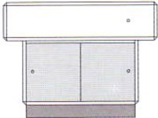
Showfront MUS 1200 / 1500 (1) 1200 L x 600 W x 900 H (2) 1500 L x 600 W x 900 H
