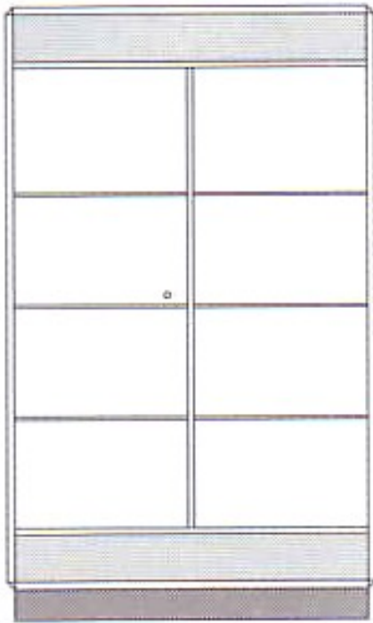
Showfront TPF 1200 / 1500 (1) 600 L x 1200 W x 2000 H (2) 600 L x 1500 W x 2000 H
