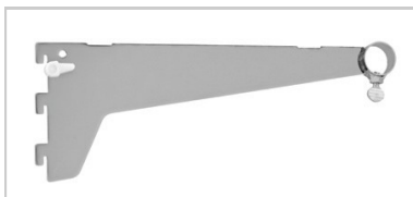
SYSTEM 40 HANGRAIL BRACKET 280MM LONG FOR 25MM TUBE CODE S1391CH COLOUR CHROME
